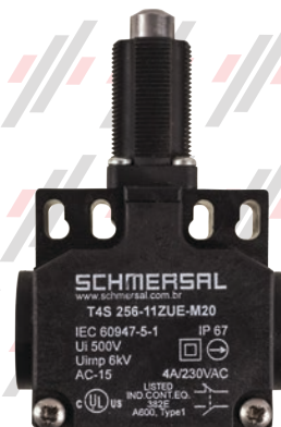
PE0100517 LIMIT SWITCH - SKIRT SWITCH LARGE BASE W/ PLUNGER
