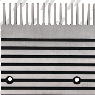
POGOA453A6 (ALUMINUM) 5 - 5/8" - 17T - 48J/UB ECALATOR
