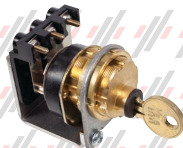
PO6410E6 KEY SWITCH RB & J ESCALATOR
