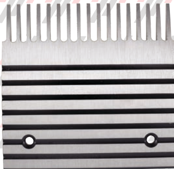
POGOA453A4 (ALUMINUM) 5 - 3/4" - 17T - 32J/UB, 44J/UB, 48J/UB ECALATOR
