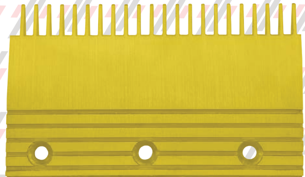
PN1200107Y (YELLOW ALUMINUM) 8" - 22T - LH - AVANTI ESCALATOR
