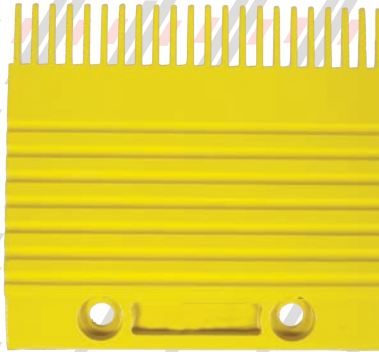
PK1200123 (YELLOW ALUMINUM) CENTER - 22T - KONE ECO ESCALATOR
