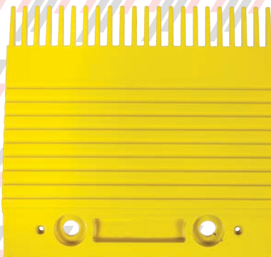
PK2209590Y (YELLOW ALUMINUM) CENTER - 22T - TYPE C - O&K RTV ESCALATOR
