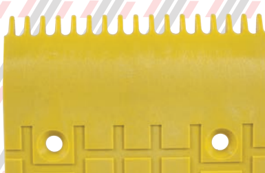
PIH2200116-17 (YELLOW PLASTIC) CENTER - 17T COMBPLATE HITACHI ESCALATOR
