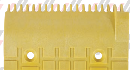
PIH2200122 (YELLOW PLASTIC) RIGHT - 19T COMBPLATE HITACHI ESCALATOR
