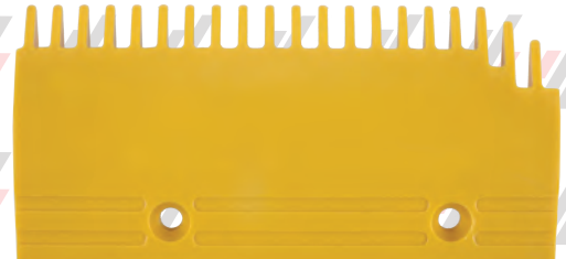
PFX129AW1 (YELLOW PLASTIC) RH - 20T - 203mm - 2 RECESSED TEETH - 2 HOLE VS1200 ESCALATOR
