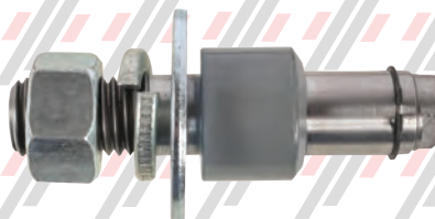
PH91237A IDLER SHAFT - LONG HAUGHTON ESCALATOR
