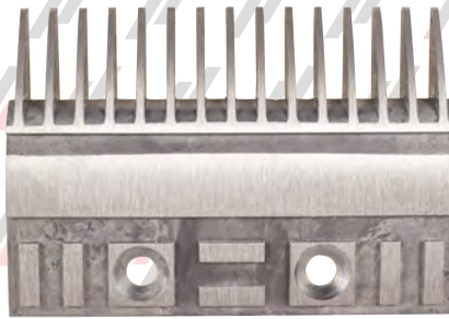
PH63108 (ALUMINUM) CENTER 4-15/16" 15T HAUGHTON ESCALATOR
