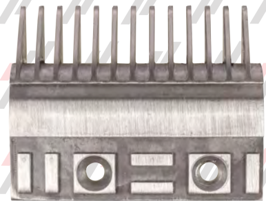
PH83085 (ALUMINUM) RH - 600mm 4-15/32" 13T HAUGHTON ESCALATOR
