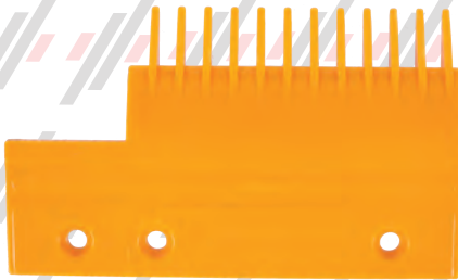
PY655B06DH05 (ORANGE PLASTIC) LH - 8" - 12T - HYUNDAI ESCALATOR
