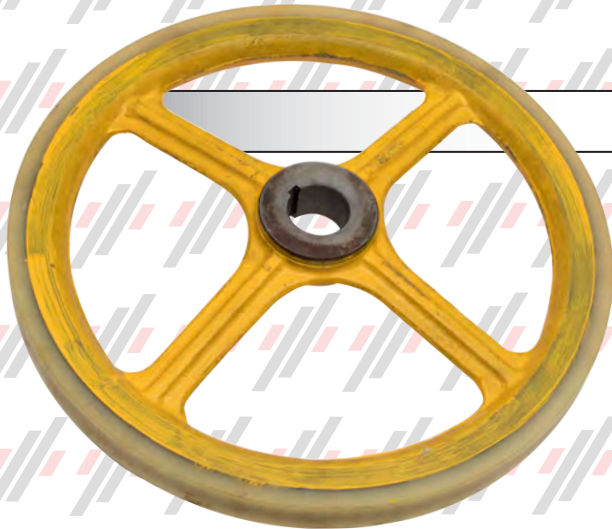
PG0600400 HANDRAIL DRIVE SHEAVE- 18" DIAMETER - LG ESCALATOR
