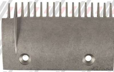
PG2L08780LD (DULL ALUMINUM) LEFT - 17T - 2 TEETH RAISED LG ESCALATOR
