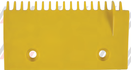
PG2L08317 (YELLOW PLASTIC) RH - 17T - 2 RAISED TEETH LG ESCALATOR
