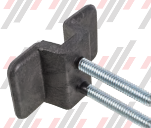
PM60440 2 BOLT GUIDE - NEWEL MONTGOMERY ESCALATOR
