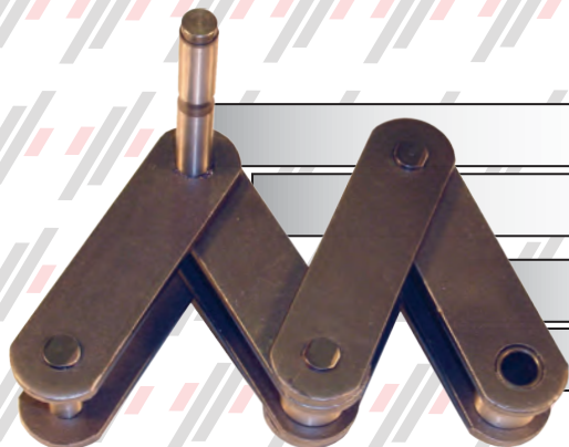
PM67883 STEP CHAIN - 1PAIR - 1 AXLE - HR ESCALATOR
