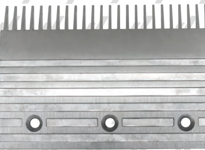
PMB32484 (ALUMINUM) CENTER - 8 3/8" W - 25T - MONTGOMERY ESCALATOR
