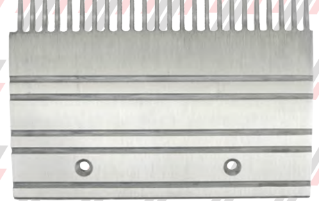
POGAA453BM5 (ALUMINUM) 205.12mm 24T - 506SL & 506NCE ESCALATOR
