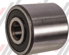
PO0800101 NEWEL BEARING 30mm OD 28mm W x 10mm ID - RB ESCALAIRES
