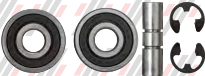
PO0800100 NEWEL BEARING ASSEMBLY R & RB ESCALAIRE
