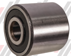
PO0800101 NEWEL BEARING 30mm OD 28mm W x 10mm ID - RB ESCALAIRE
