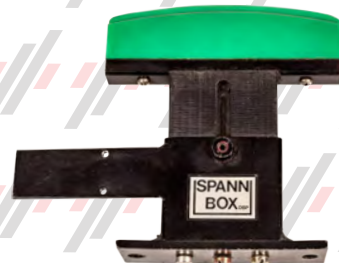
PO0600802 SWITCH BROKEN CHAIN - 506NCE ESCALATOR
