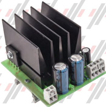
PSSSG897220 POWER SUPPLY BOARD 9300 ESCALATOR
