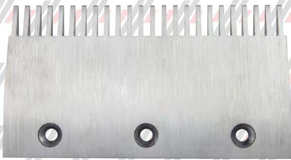
PN1200101 (ALUMINUM) 8" - 24T - VELINO ESCALATOR
