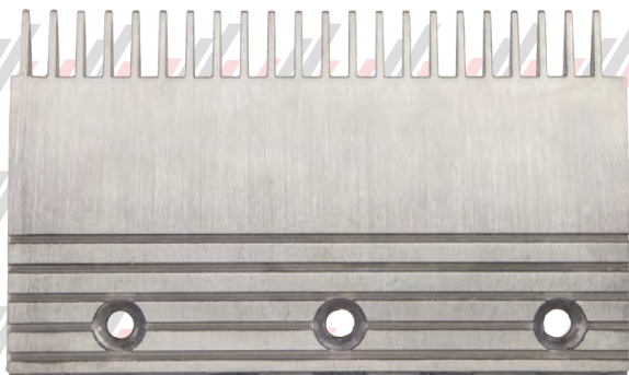
PN1200109 (ALUMINUM) 8" - 22T - RH - AVANTI ESCALATOR
