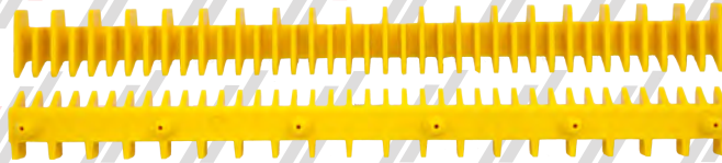
PN1000700 (YELLOW PLASTIC) DEMARICATION - CENTER LONG - THYSSEN ESCALATOR
