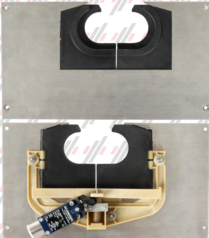
PW0100305 HR ENTRY DEVICE - LH - MOD ESCALATOR
