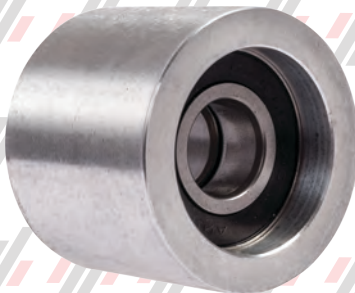
PW5193D65H01 ROLLER - BROKEN BELT SWITCH - SINGLE BELT MODULAR ESCALATOR
