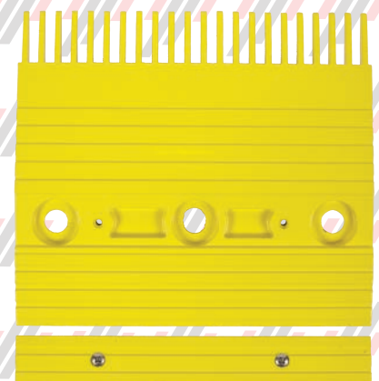
PK1718892Y (YELLOW ALUMINUM) RH - 22T - O&K ESCALATOR
