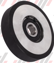
PK0900201 ROLLER - STEP TRAIL - 100mm OD - 21mm WIDE 17mm BORE - O&K ESCALATOR
