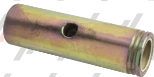
PK1000650 STEP CONNECTION AXLE- 13mm ID 4.25" OAL - ECO3000 ESCALATOR
