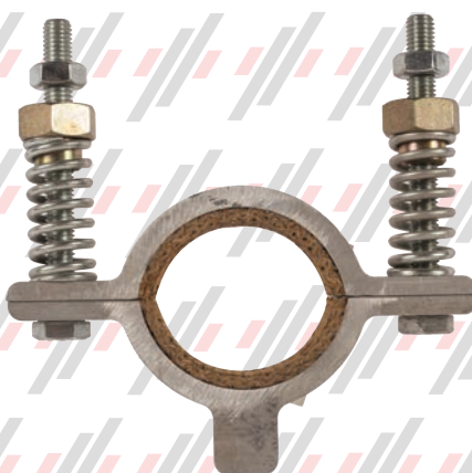
PFC65077001 60mm LEVER ASSEMBLY FUJITEC ESCALATOR
