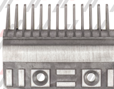
PH83085 (ALUMINUM) RH - 600mm 4-15/32" 13T HAUGHTON ESCALATOR
