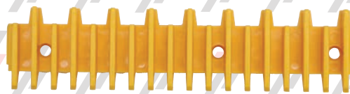
PY645B028H02Y (YELLOW PLASTIC) CENTER- 163.8mm BOLT THROUGH STYLE HYUNDAI ESCALATOR
