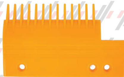
PY655B06DH04 (ORANGE PLASTIC) RH - 8" - 13T - HYUNDAI ESCALATOR
