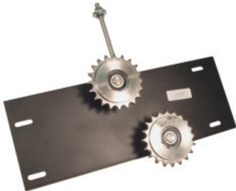
OTIS HANDRAIL IDLER SPROCKET #60 CHAIN 20 TEETH
